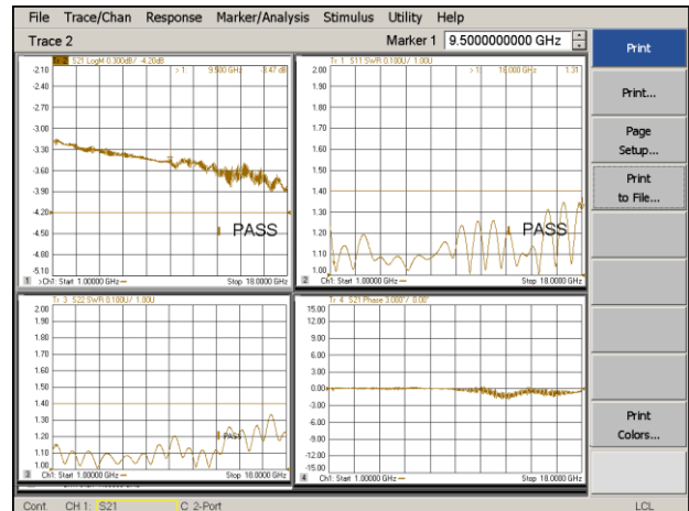
The test curve of output2
