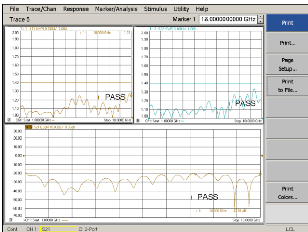
The test curve of isolation
